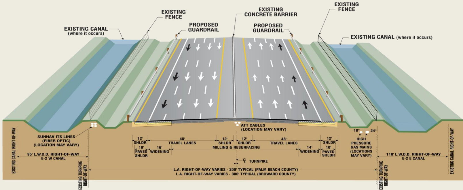
PROPOSED TYPICAL SECTION SAWGRASS EXPRESSWAY TO ATLANTIC AVENUE
